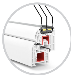
T-Classic Plus Innovative Form 8 Kammern Uw 0,75 W/m²K
