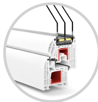
T-Classic Plus Innovative Form 8 Kammern
